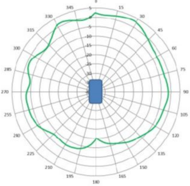
6.5 GHz Wi-Fi (R2) Average Elevation 0 6.5 GHz Antenna Average Elevation 0
