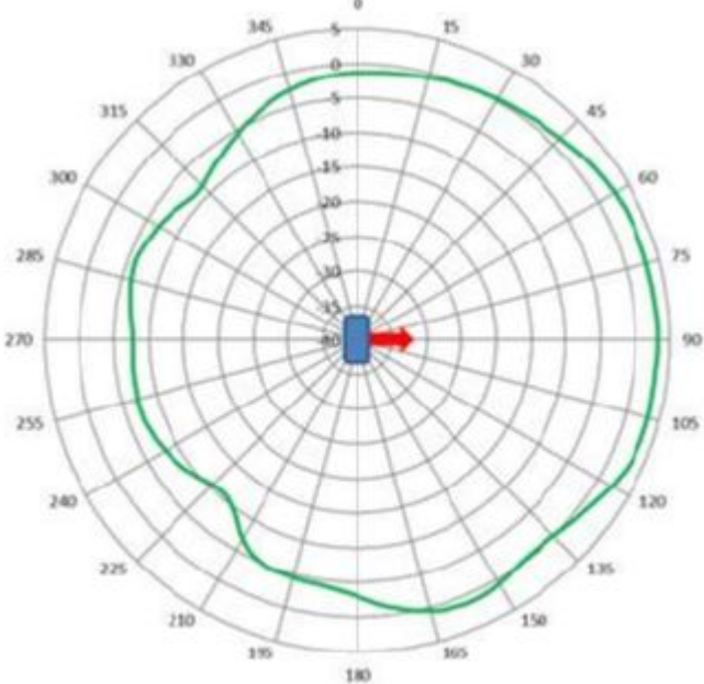
6.5 GHz Wi-Fi (R2) Average Azimuth 6.5 GHz Antenna Average Azimuth
